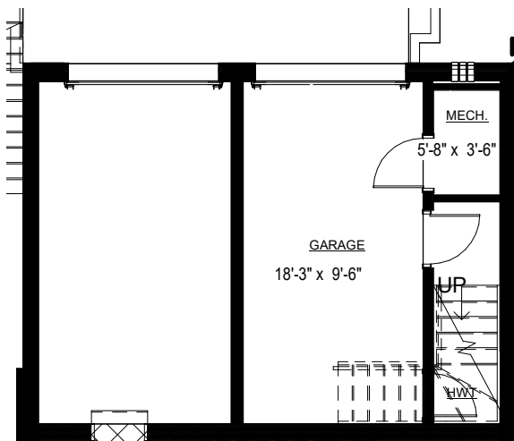
GARAGE / LOWER LEVEL MECH. SPACE
