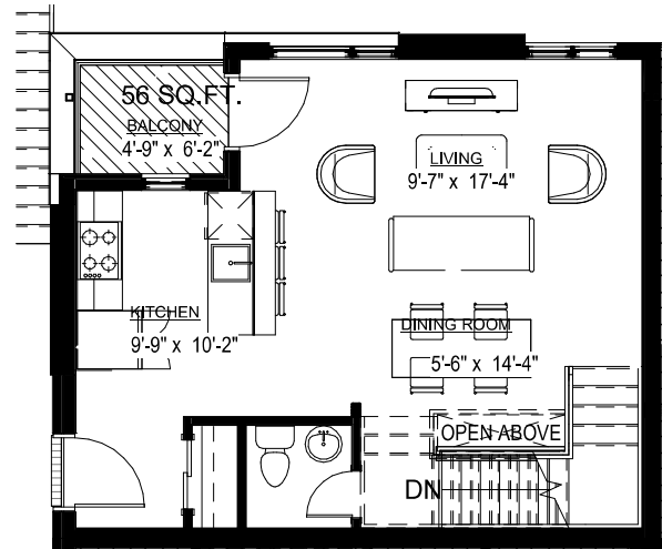
1ST LEVEL 516 SQ.FT.
