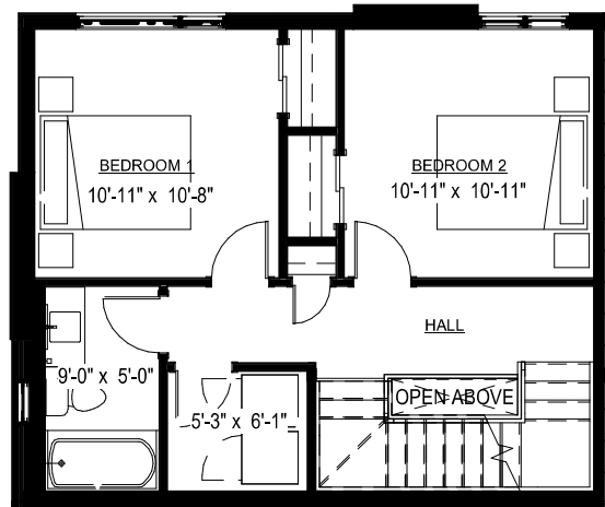
2ND LEVEL 556 SQ.FT.
