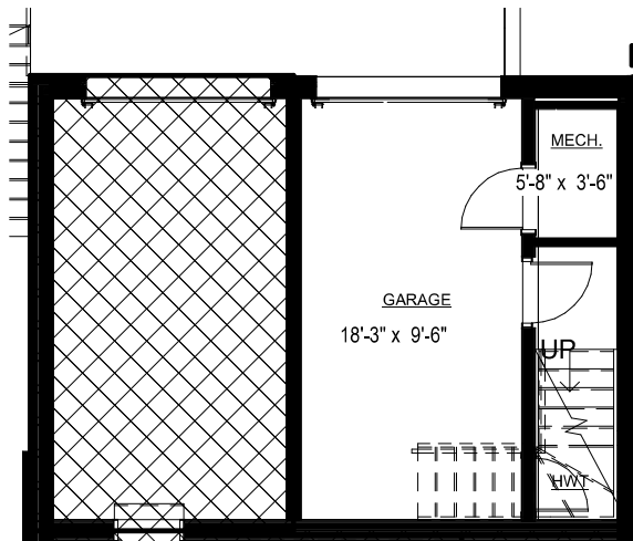
BASEMENT / GARAGE 285 SQ.FT.
