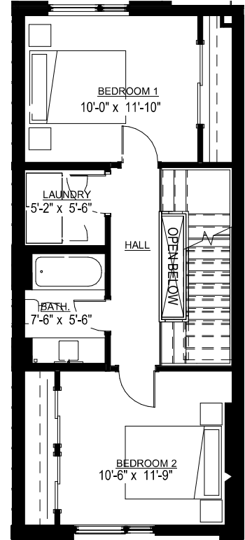
556 SQ.FT. 2ND LEVEL
